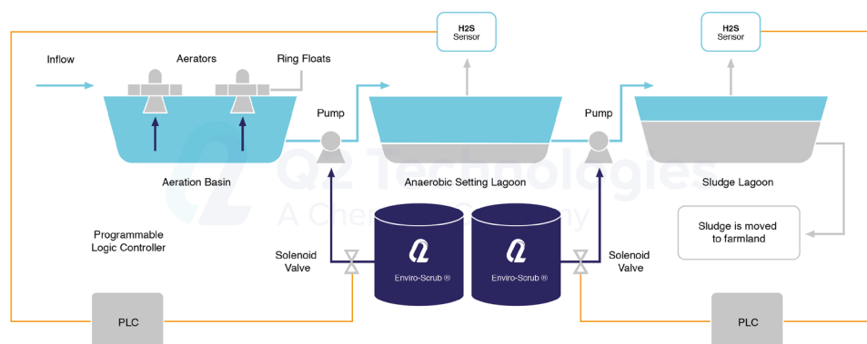
DIAGRAM 1. SLUDGE TREATMENT FOR FOOD PROCESSOR
